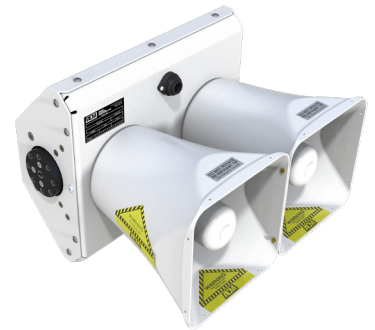
LS600 Speaker
